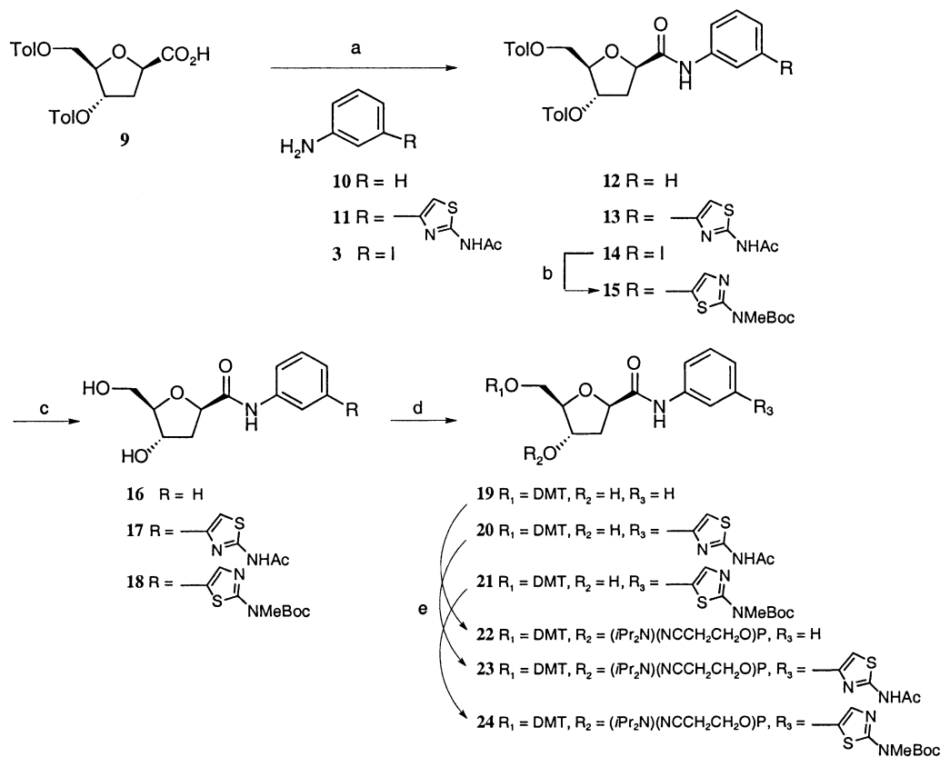
Scheme 2. Synthesis of phosphoramidites 22 , 23 and 24 . Reagents and reaction conditions: (a) chloromethylpyridinium iodide, Et 3 N, CH 2 Cl 2 , 60 °C (90–95%); (b) 5 , Pd(Ph 3 ) 4 , DMF, 60 °C (92%); (c) NaOMe, MeOH (91–97%); (d) DMTCl, Et 3 N, DMF (80%); (e) CIP(OCH 2 CH 2 CN)(NiPr) 2 , N,N -diisopropylethylamine, CH 2 Cl 2 (63–80%).
