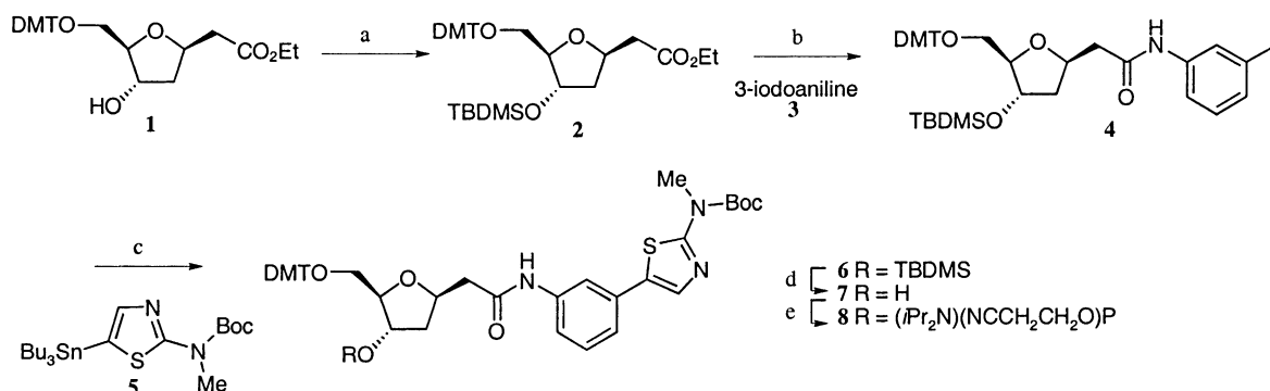
Scheme 1. Synthesis of phosphoramidite 8 . Reagents and reaction conditions: (a) TBDMSCl, imidazole, DMF (85%); (b) AlMe 3 , molecular sieves 4 Å, toluene, (90%); (c) 5 , Pd(Ph 3 ) 4 , DMF, 60 °C (87%); (d) Bu 4 NF, THF (87%); (e) CIP(OCH 2 CH 2 CN)(NiPr) 2 , N,N -diisopropylethylamine, CH 2 Cl 2 (61%).
