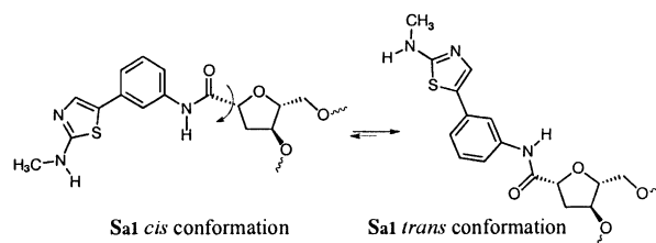
Figure 2. trans and cis conformations of compound S a1 .
