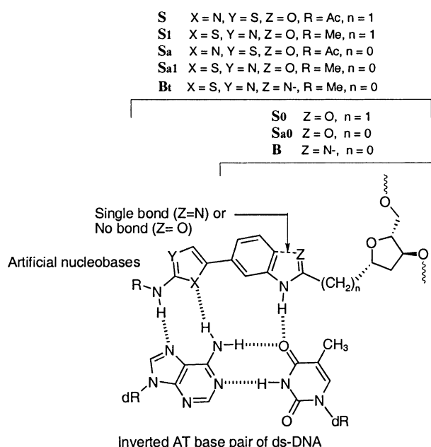
Figure 1. Structure of the artificial nucleobases and proposed model for their specific recognition of an inverted A•T base pair.
